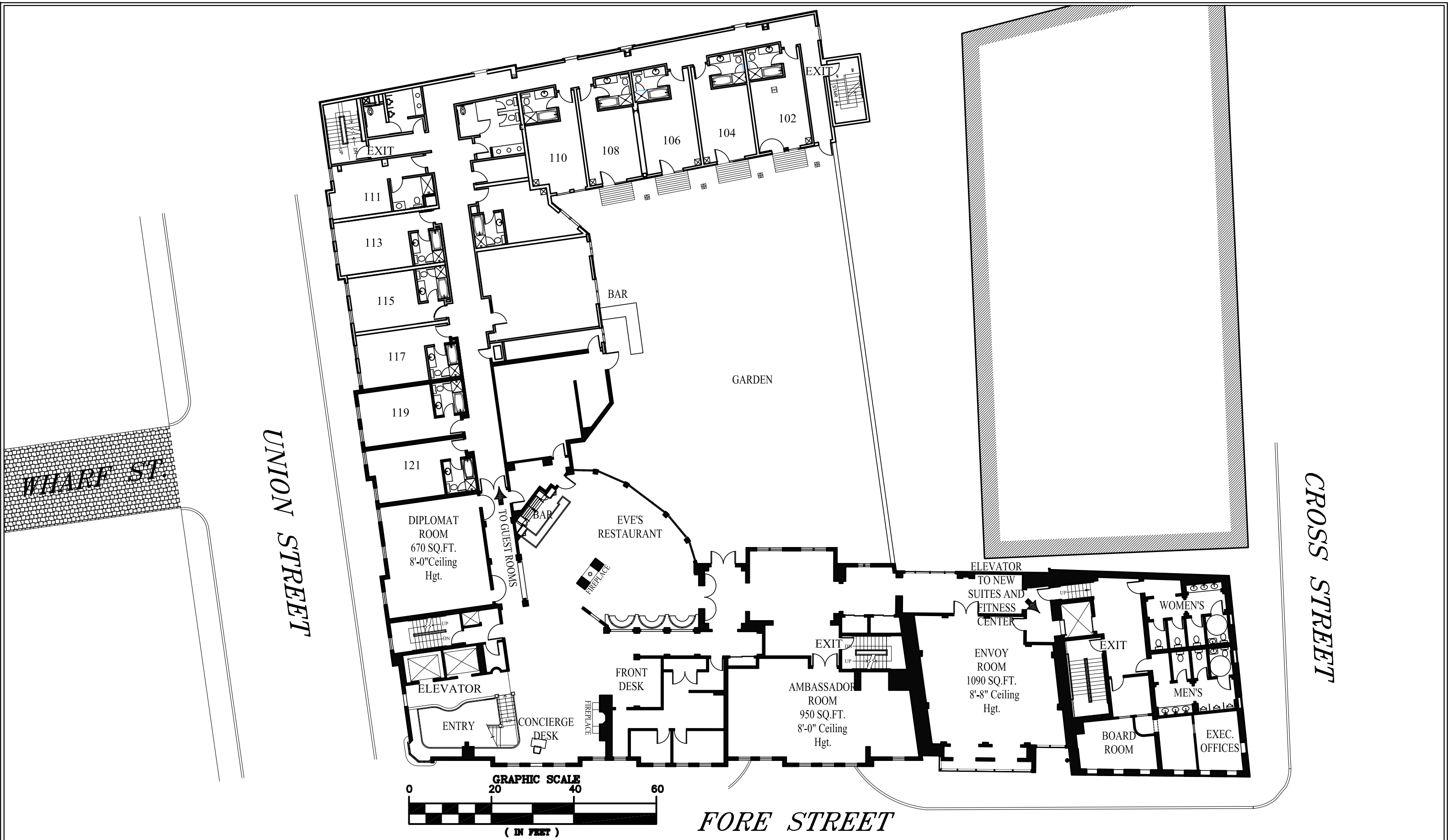
PORTLAND HARBOR HOTEL FIRST FLOOR LEVEL
